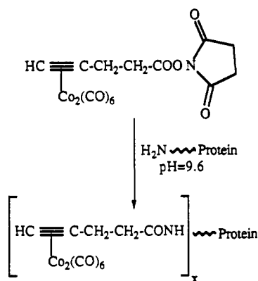
Scheme II
